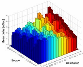
Figure 3: Mean flows delay in the homogeneous system.
